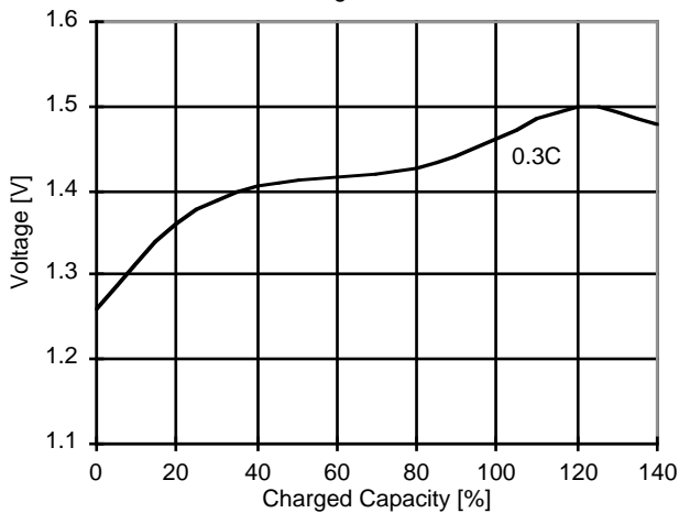
Charge @ 20°C
