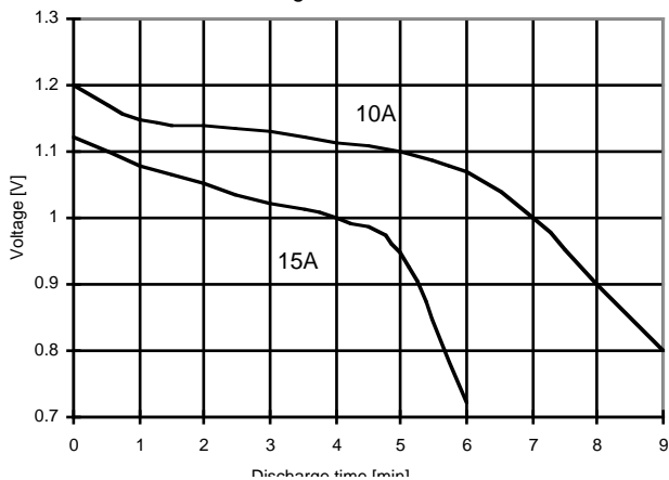
Discharge at low rate @ 20°C
