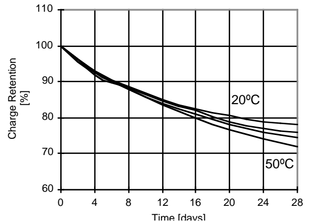
Charge Retention
