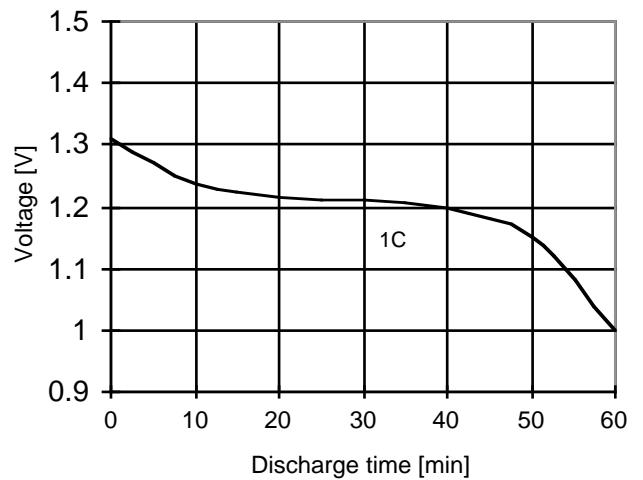
Discharge at @ 20°C
